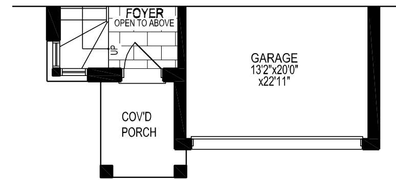
PART. MAIN LEVEL STYLE B
